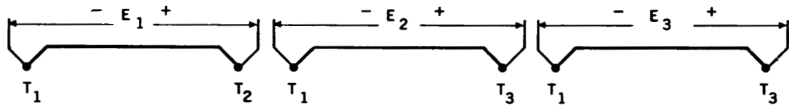
Fig 21 Thermocouple EMF—Temperature Relations
