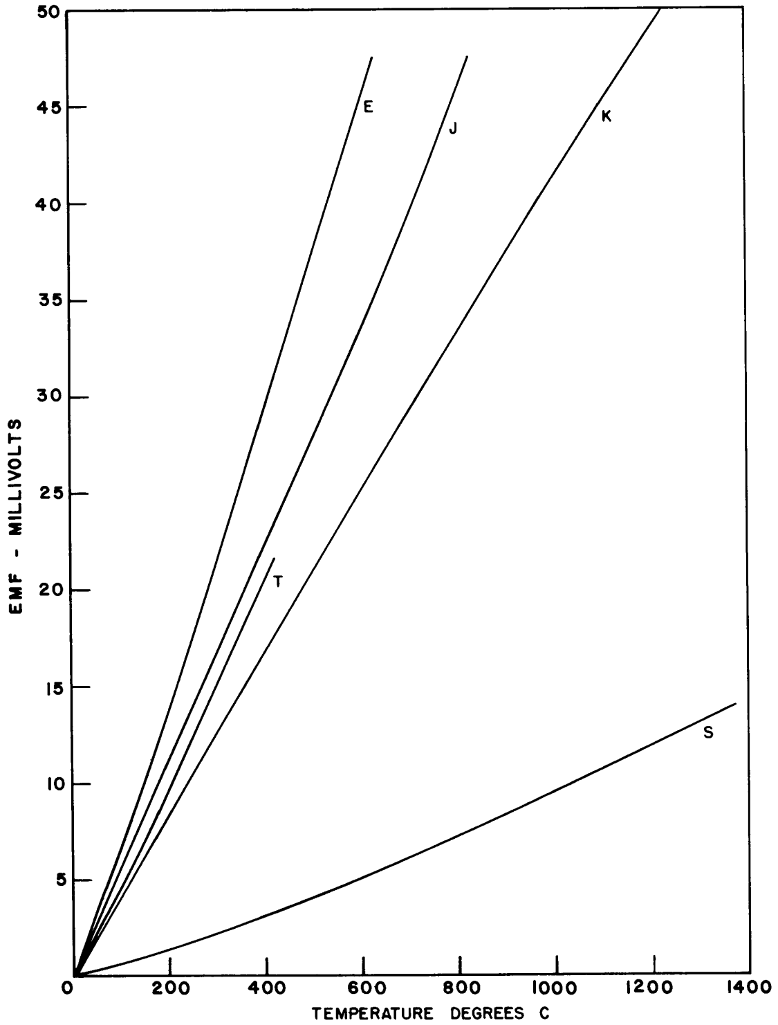
Fig 20 Thermocouple EMF Versus Temperature for Various Thermocouple Materials (Reference Temperature = 0°C)
