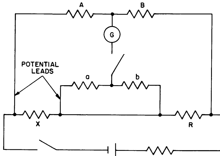
Fig 37 Kelvin Bridge Circuit
