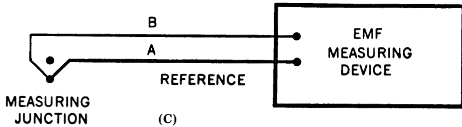
Fig 22 Thermocouple Circuits
