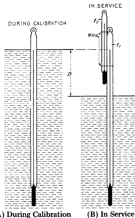
Fig 9 Thermometer Calibrated for Total Immersion and Used for Partial Immersion
