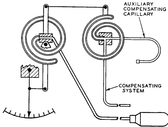
Fig 11 Fully Compensated Liquid, Mercury, or Gas Filled Thermal System
