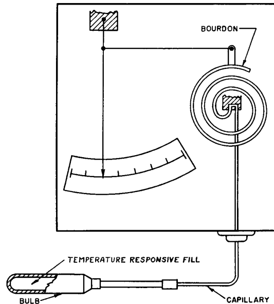
Fig 10 Filled-System Thermometer
