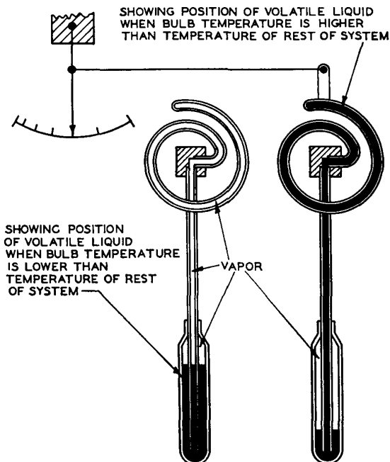
Fig 15 Vapor Pressure Thermal System, Class IIC (For Use Where T_m < T_a or > T_a )
