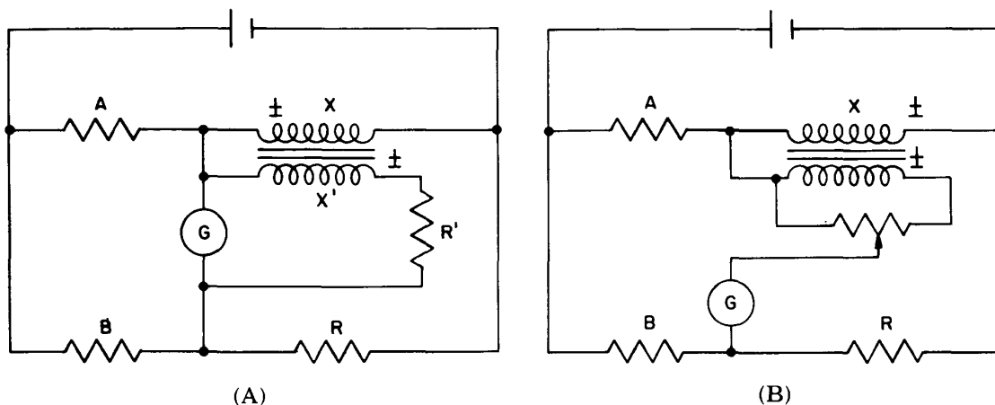
Fig 43 Compensation of Wheatstone Bridge for Inductive Effects
