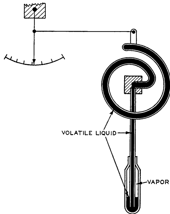
Fig 13 Vapor Pressure Thermal System, Class IIA (For Use Where T_m > T_d )
